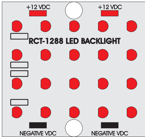
Viewed with Tyco Connector Plug-In Face Down.
