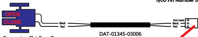
Mate-N-Loc Connector, Flat Face Down 2 Pin Part Number 1-480698-0
