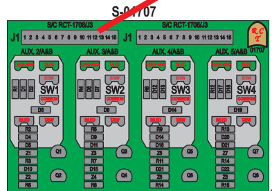
Viewed with Tyco Connector Plug-In Face Down.
