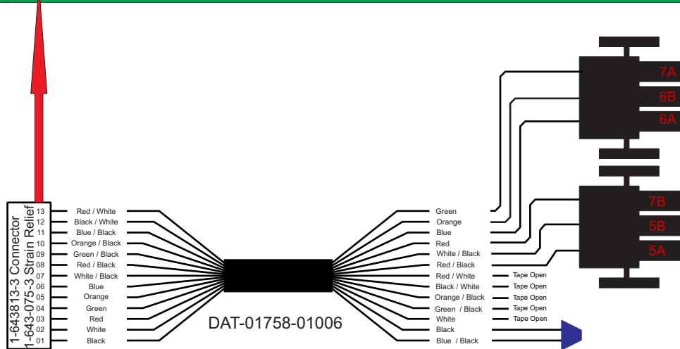
Viewed with Tyco Connector Plug-In Face-Down.
