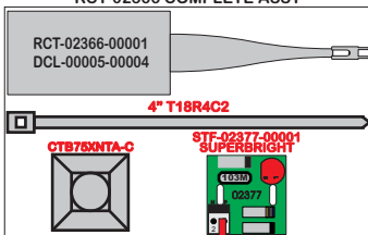
RCT-02366 COMPLETE ASSY
